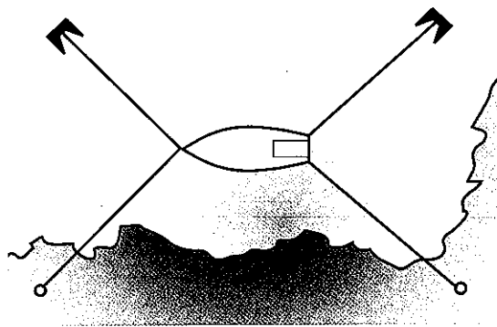
One of many possible arrangements that can be used to secure a boat in a hurricane hole.
